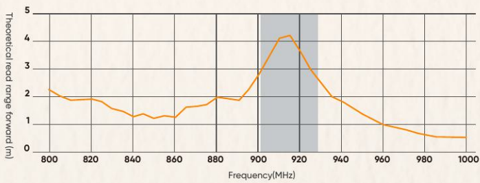
Reading Range Under Different Frequency-FCC Standard
