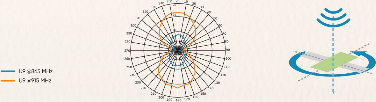
Orientation Sensitivity
